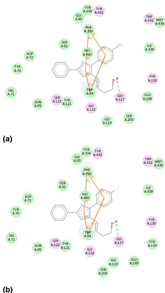
Figure 4: 2D depiction of interactions of compounds (a) 3d and (b) 3i with active site of AChE
